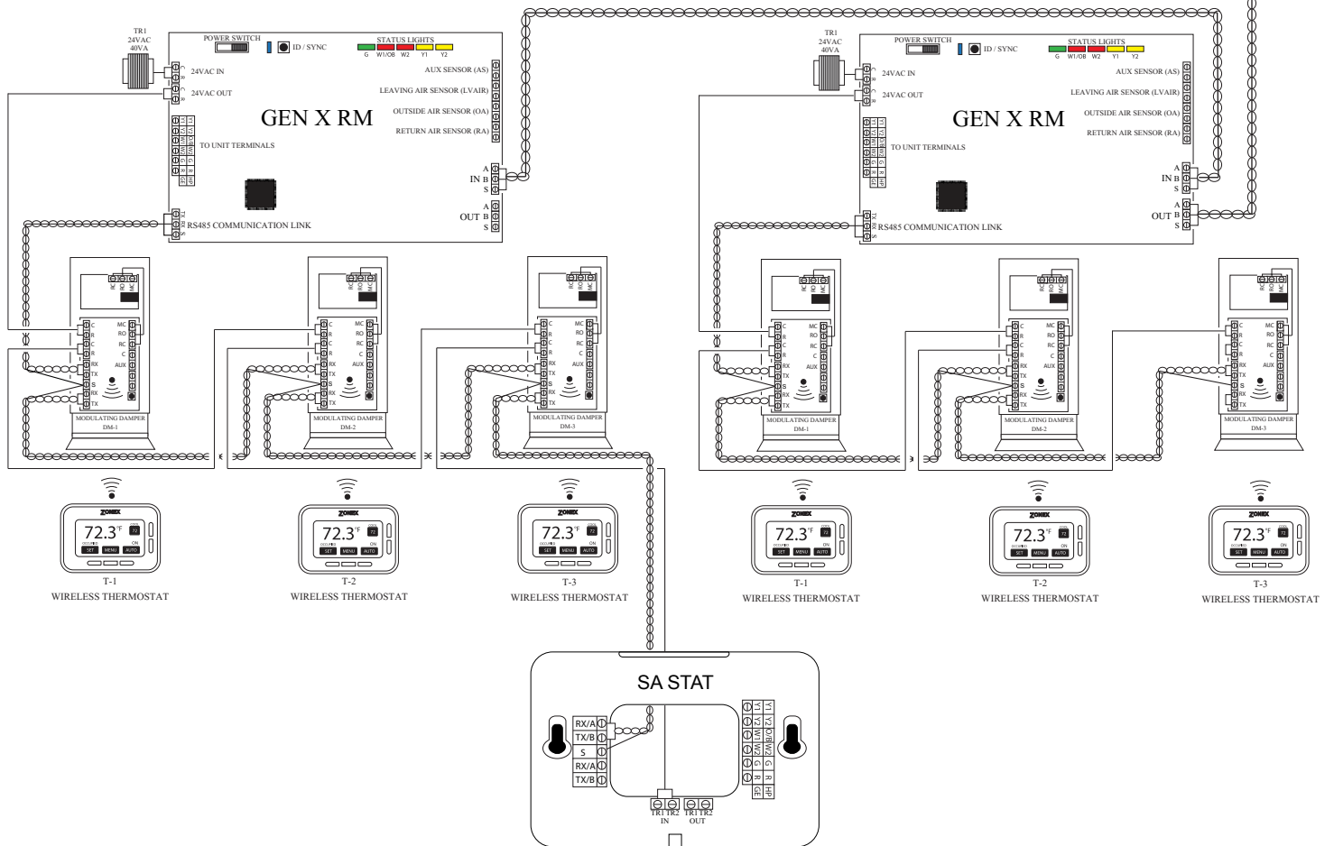
T-1 WIRELESS THERMOSTAT
